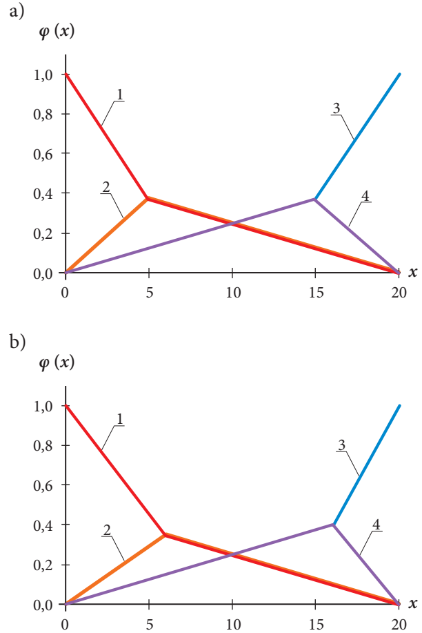
Fig. 5. Current distribution functions for the symmetric (a) and asymmetric (b) parallel power scheme
