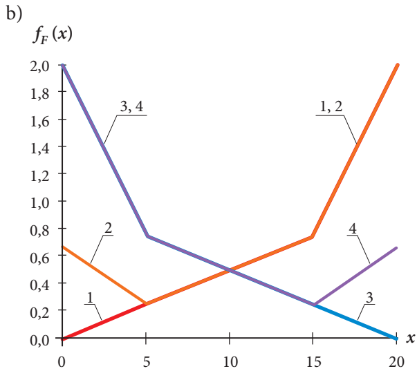
Fig. 8. Resistance functions for the feeders of symmetric (a) and asymmetric (b) parallel power scheme
