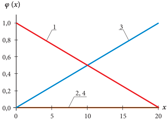
Fig. 3. Current distribution functions for the feeders of traction substation in case of two-way power scheme
