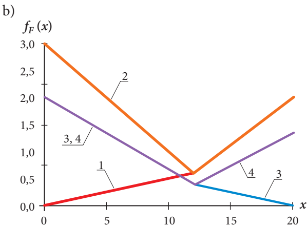
Fig. 7. Resistance functions for the feeders of symmetric (a) and asymmetric (b) nodal power scheme
