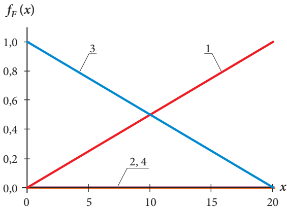
Fig. 6. Resistance functions for the feeders of two-way power supply scheme
