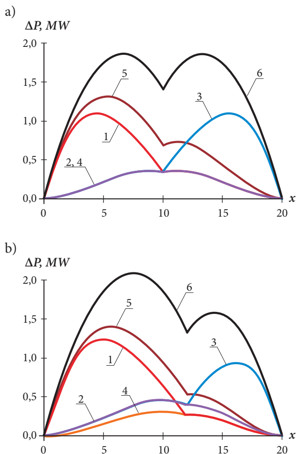
Fig. 10. Power losses for the symmetric (a) and asymmetric (b) nodal power supply scheme: 1–4) the components appropriate to the feeders of traction substations, 5) losses that account for a substation, 6) total power losses in the traction network
