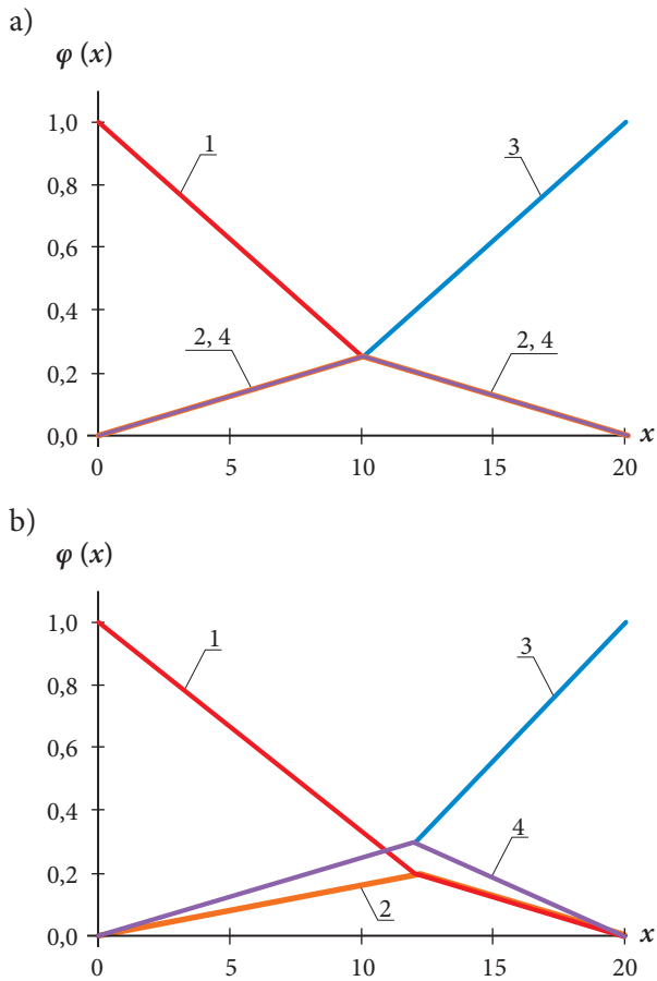
Fig. 4. Current distribution functions for the feeders of the nodal power scheme: a) symmetric, b) asymmetric
