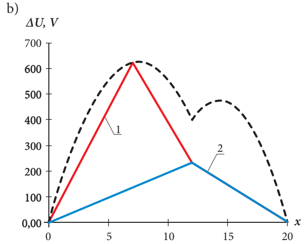
Fig. 9. Voltage distribution functions for the symmetric (a) and the asymmetric (b) nodal power supply scheme: 1) on the passing track, 2) on the adjacent track
