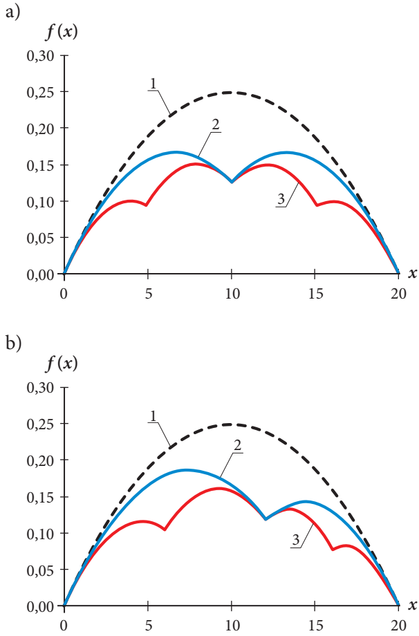
Fig. 2. Graphical representation of functions of resistance for symmetric (a) and asymmetric (b) power schemes: 1) two-way power scheme, 2) nodal, 3) parallel
