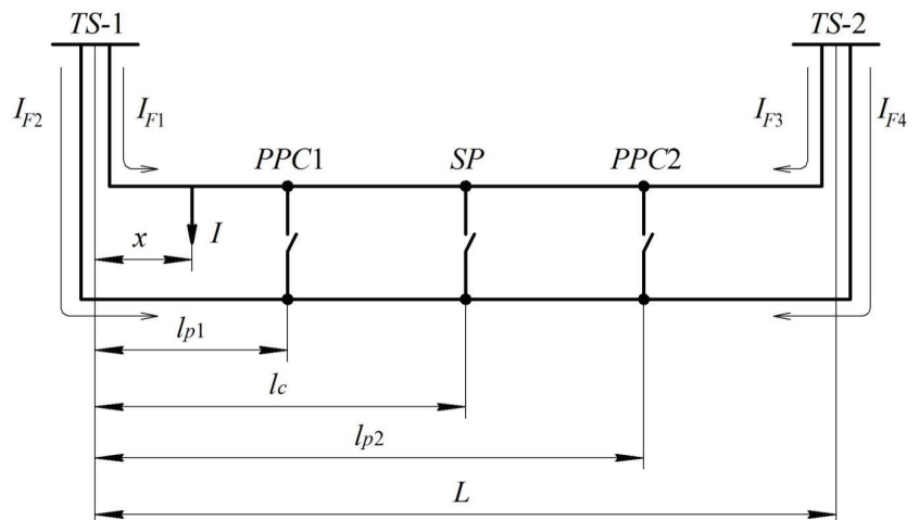
Fig. 1. Generalized computational scheme of traction substations zone
