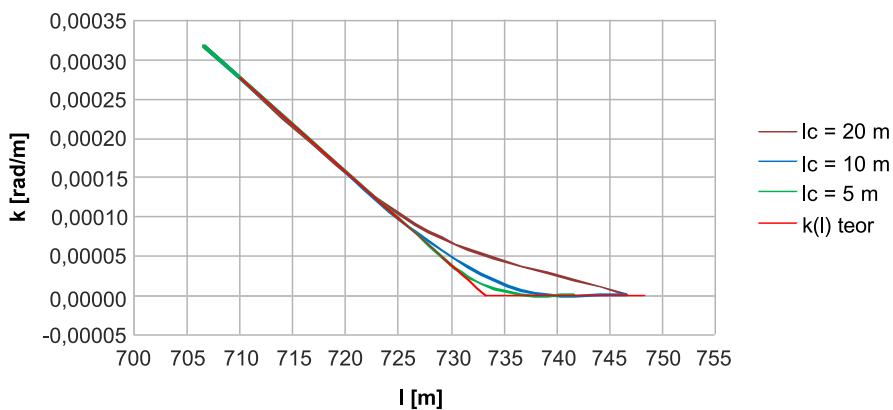
Fig. 7. Plot of the curvature ordinates k(l) theor in the section of transition from transition curve in the form of a clothoid to a straight section (variant I) for the assumed lengths of the moving chord l_c = 5 m, 10 m and 20 m ( \alpha = \pi/4 rad, R = 800 m, clothoid l_k = 105 m) [author's study]
