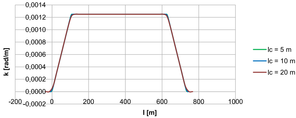
Fig. 3. Plot of the curvature ordinates k(l) in variant I for the assumed lengths of the moving chord l_c = 5 m, 10 m and 20 m ( \alpha = \pi/4 rad, R = 800 m, clothoid l_k = 105 m) [author's study]
