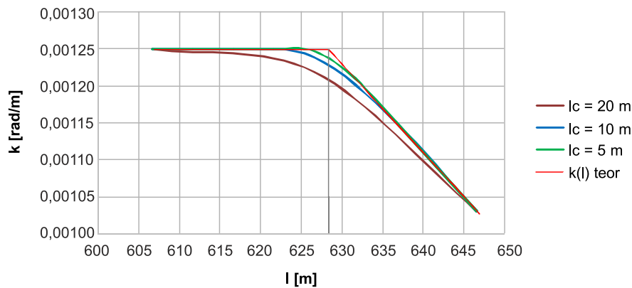
Fig. 6. Plot of the curvature ordinates k(l) theor in the section of transition from circular arc to transition curve in the form of a clothoid (variant I) for the assumed lengths of the moving chord l_c = 5 m, 10 m and 20 m ( \alpha = \pi/4 rad, R = 800 m, clothoid l_k = 105 m) [author's study]
