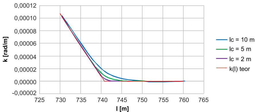
Fig. 13. Plot of the curvature ordinates k(l) theor in the section of transition from the new transition curve to a straight line (variant III) for the assumed lengths of the moving chord l_c = 2 m, 5 m and 10 m ( \alpha = \pi/4 rad, R = 800 m, l_k = 135 m) [author's study]
